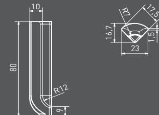
sokl vnitřní roh | TSIRH... | 23x80x10 mm cove skirting inside corner | TSIRH... | 23x80x10 mm
